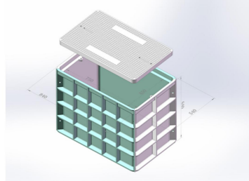
1 ▶ Telecom Manhole Chamber Product Dimension.
