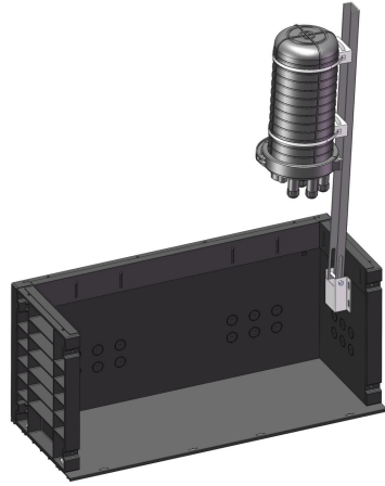
Optional-1 FOSC Fixed Frame
